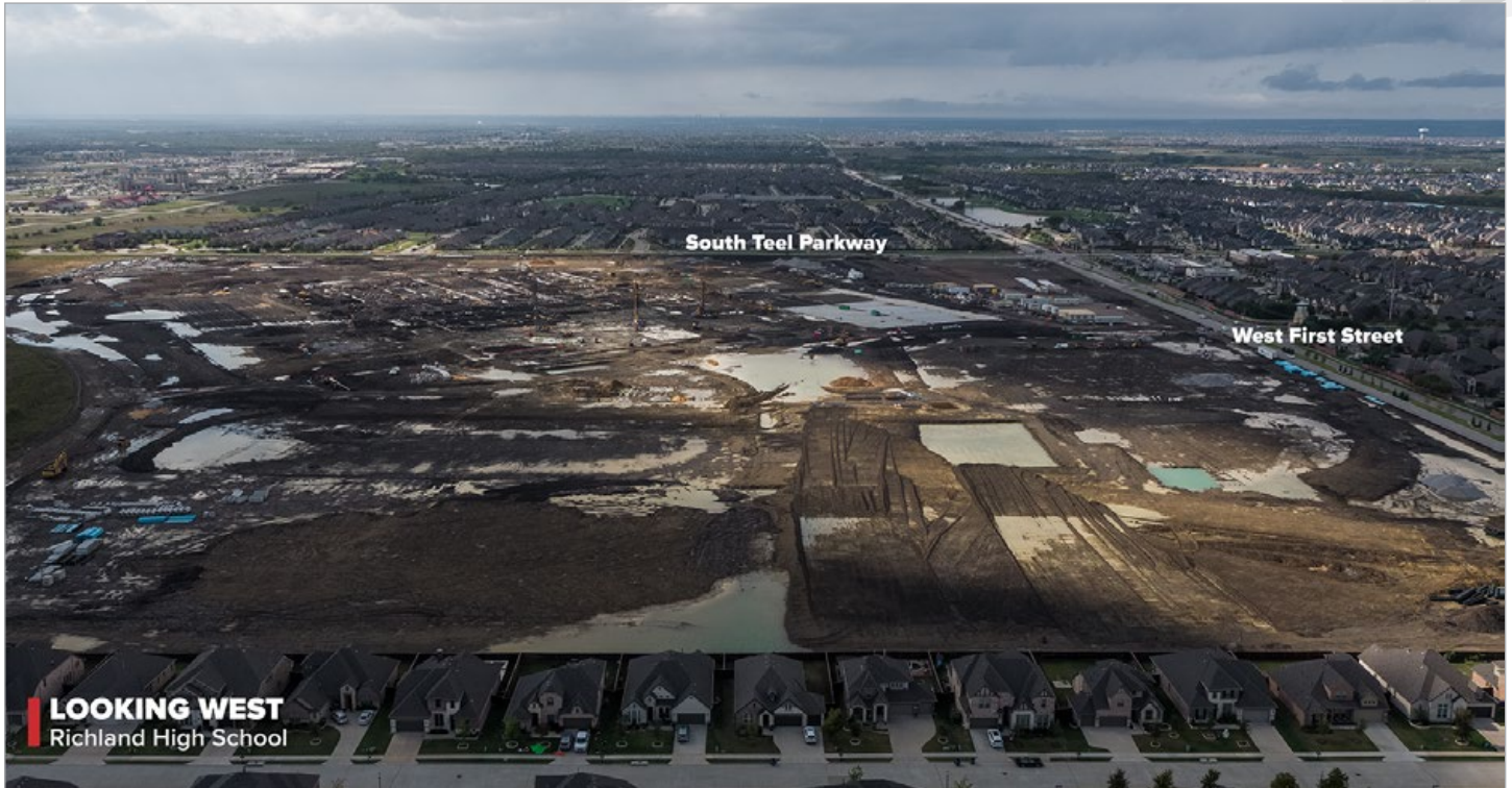
Auger Cast Pile Installation
